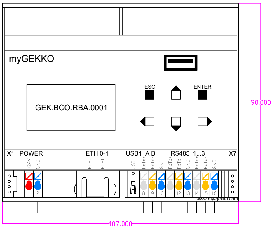
BASE R07 REG Controller X6 | 3R | 2 ETH | USB T:62mm
