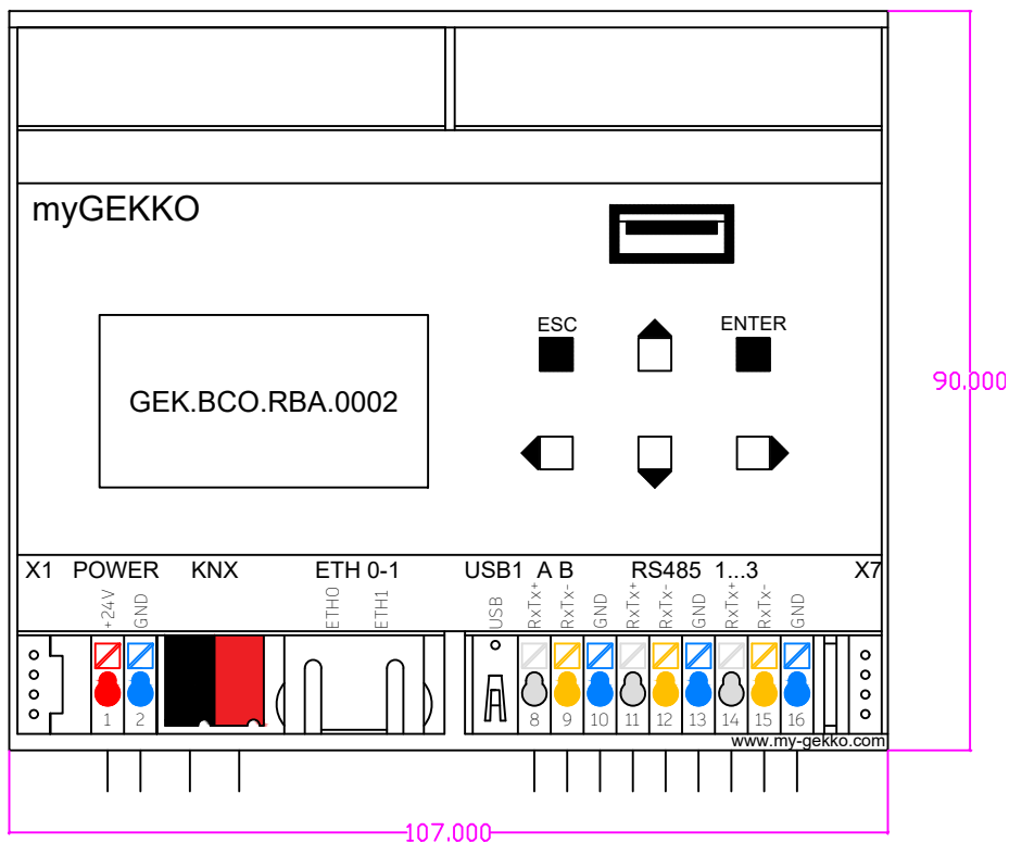
BASE R08 REG Controller X6 | 3R | 2 ETH | USB | KNX T:62mm
