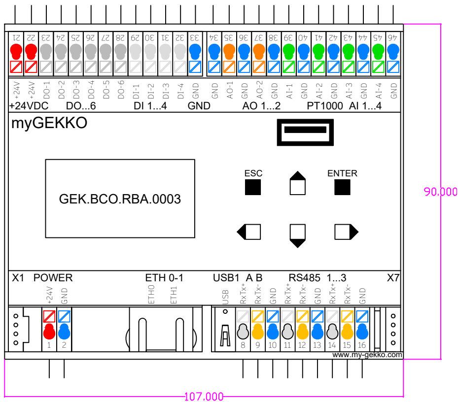
BASE R23 REG Controller X6 | 3R | 2 ETH | USB | 16IO T:62mm
