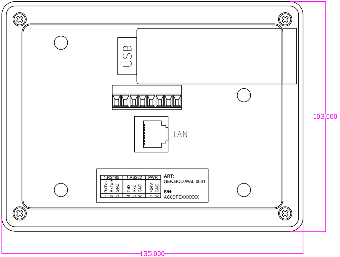
PICO W04 WALL X8 | RS232 | RS485 | ETH | USB T:21mm
