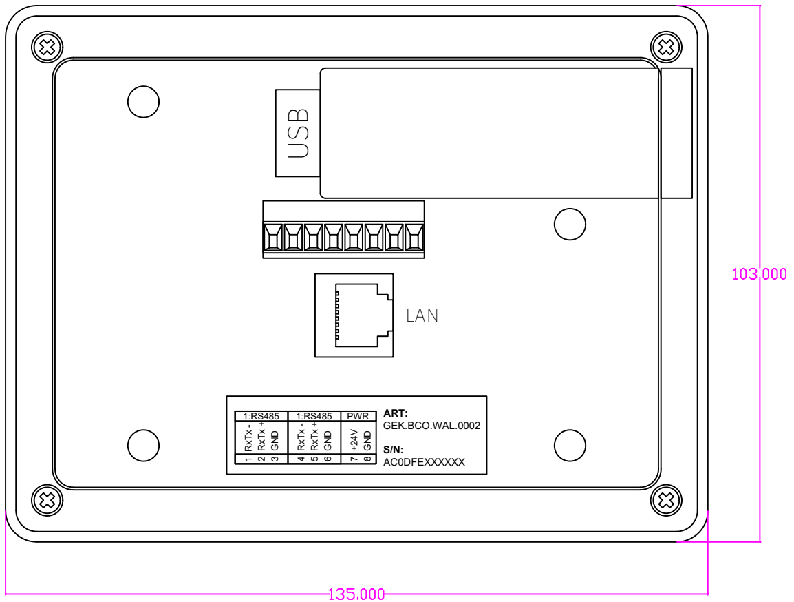
PICO W03 WALL X8 | RS232 | RS485 | ETH | USB T:21mm
