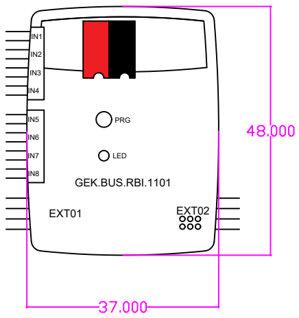
RBI11 RAUMBUS Taster Interface T:18mm
