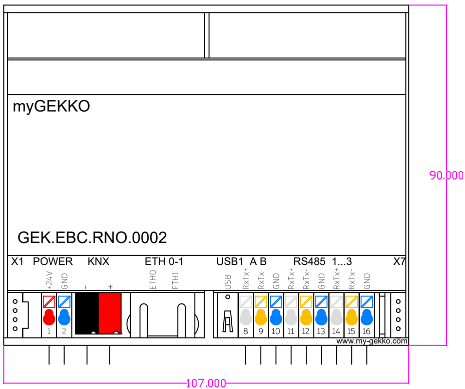
myGEKKO NODE R08 T:62mm REG 6TE
