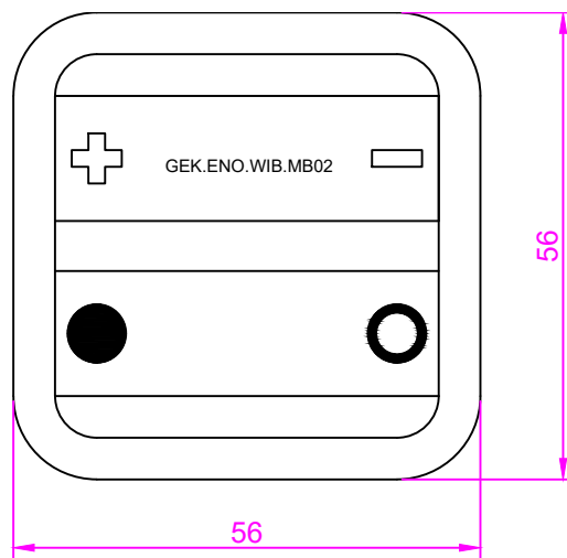
myGEKKO EnOcean Soft Button 4F, Batterielos T:21mm
