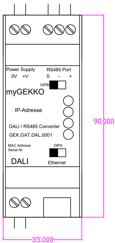
DALI / RS485 - Gateway myGEKKO Optimized T:60mm
