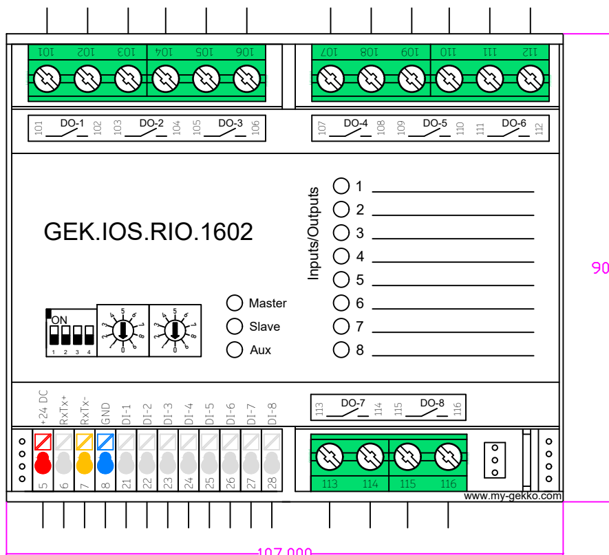
myGEKKO RIO 16s T:62mm REG 6TE
