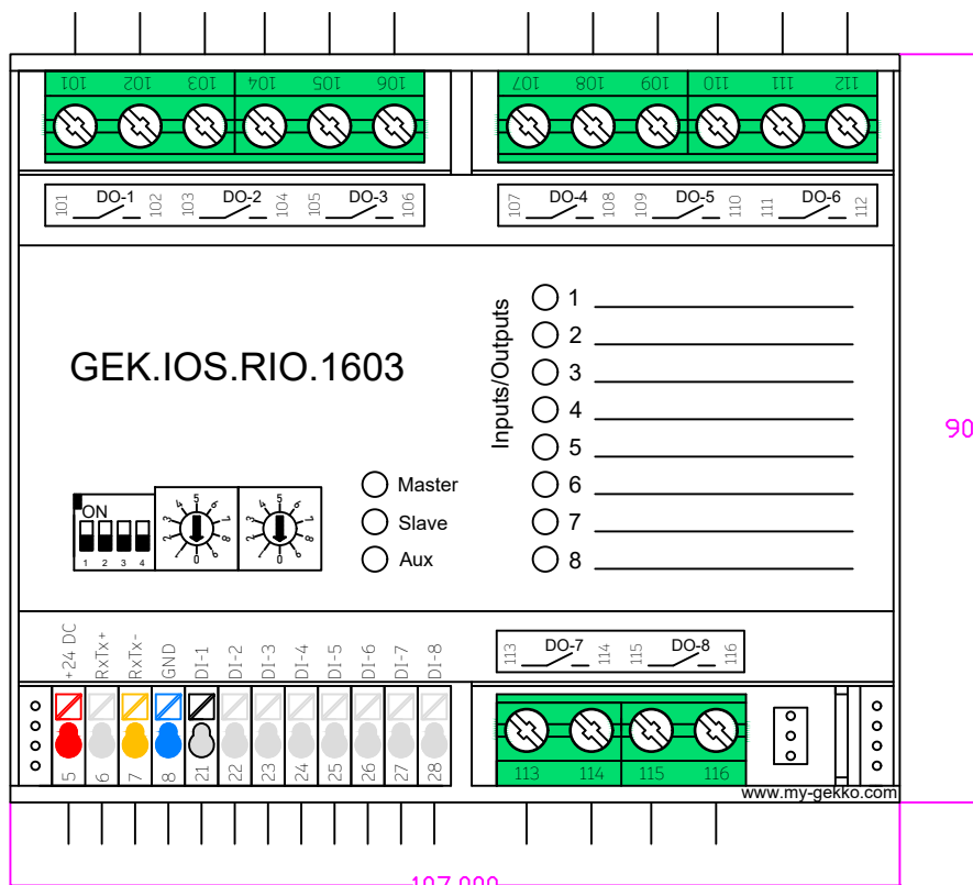
myGEKKO RIO 16sLED T:62mm REG 6TE
