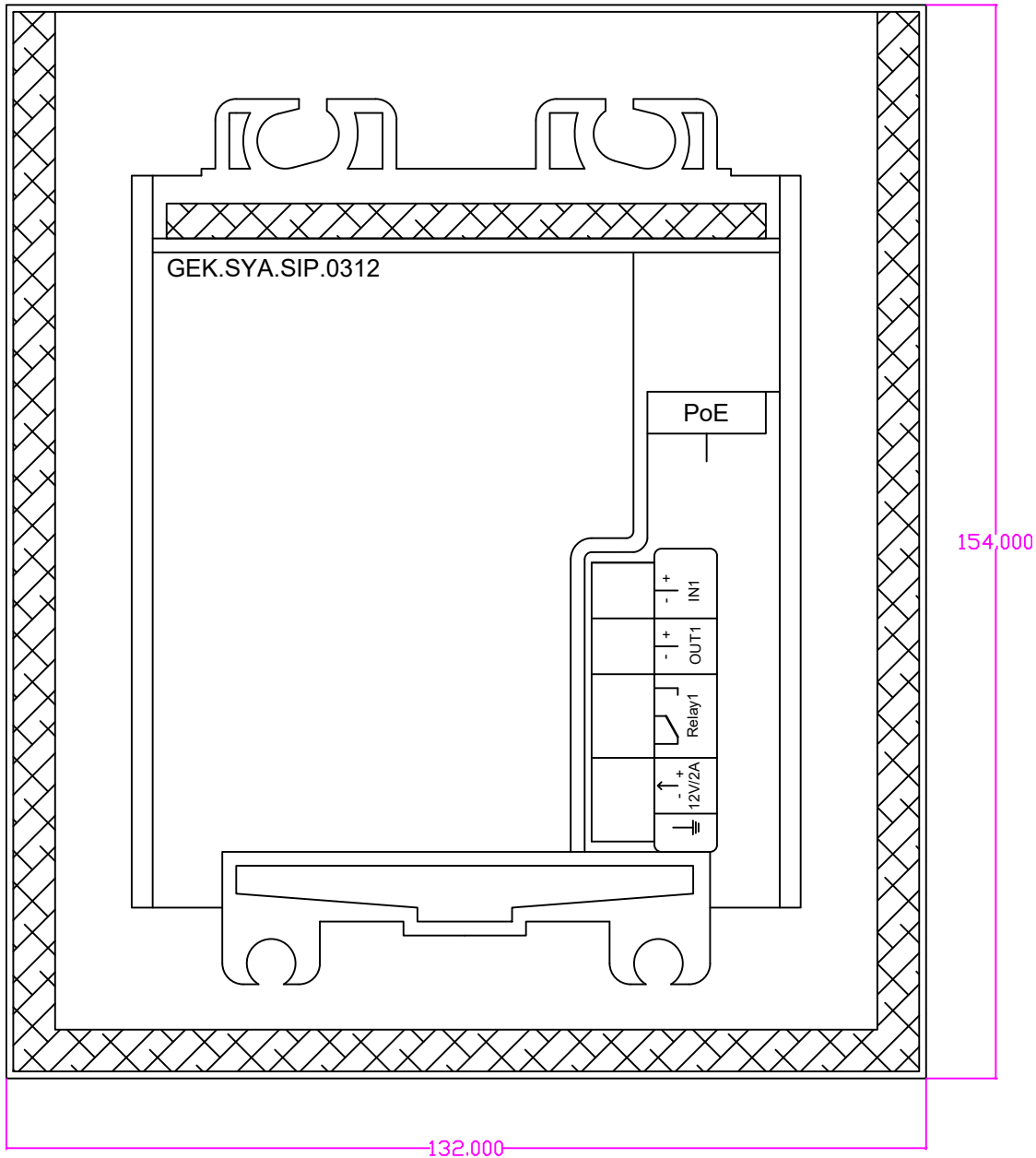
SIP03 Design Intercom IP Unterputz T:7mm
